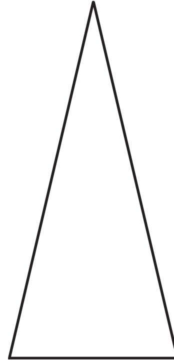
isosceles triangle
