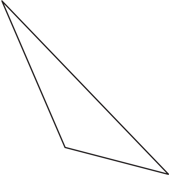
scalene triangle
