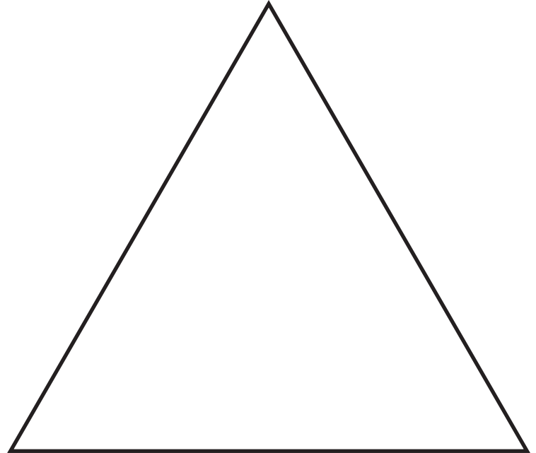
equilateral triangle
