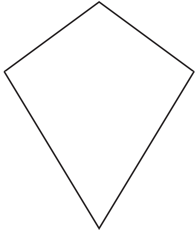
kite
