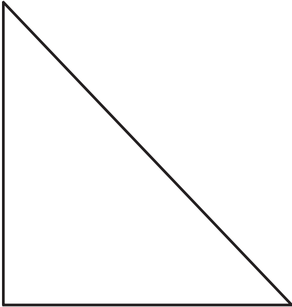
right triangle
