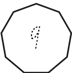
nonagon
