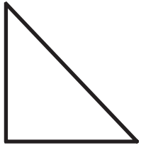
right triangle
