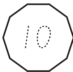
decagon
