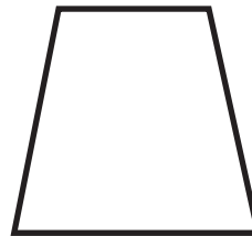
trapezoid
