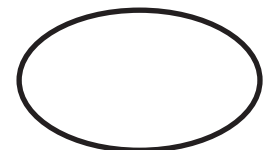
ellipse
