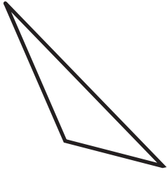
scalene triangle
